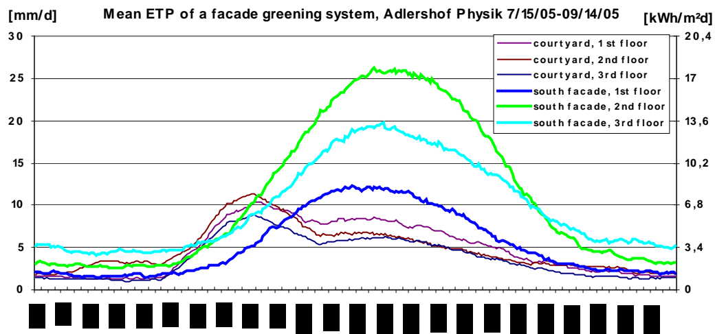
Figure 14: Mean evapotranspiration of the façade greening system in mm/day and correspondent cooling rates
