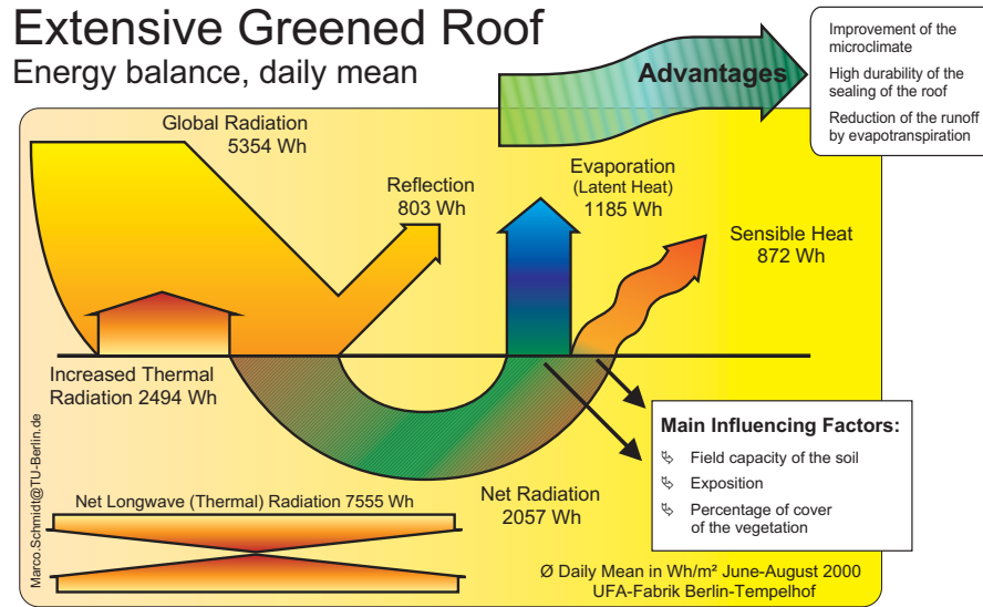
Figure 5: Extensive green roofs transfer 58% of net radiation into evapotranspiration during the summer months, UFA Fabrik in Berlin, Germany (Schmidt, 2005)
