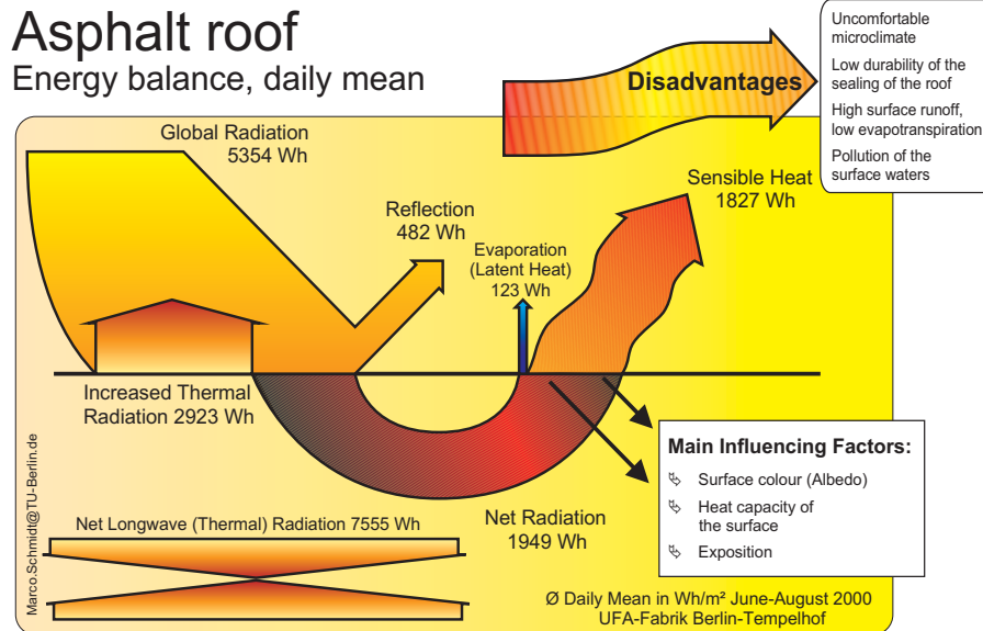
Figure 4: Radiation balance of a black asphalt roof as an example for urban radiation changes (Schmidt, 2005)
