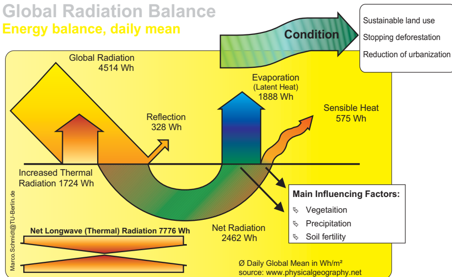
Figure 1: Global daily radiation balance as annual mean (Schmidt et al., 2007). Energy data based on www.physicalgeography.net
