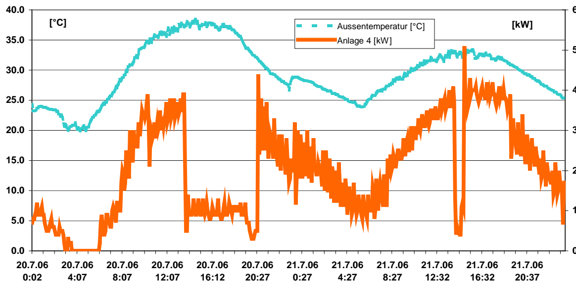
Figure 13: Evaluation of the reduction in energy consumption when switching the evaporative cooling system on and off
