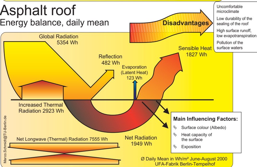
Fig. 1: Global daily radiation balance as annual mean (after: www.physicalgeography.net)
